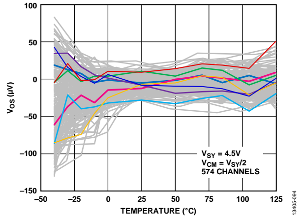
Figure 90. Input Offset Voltage ( V_{OS} ) vs. Temperature, V_{SY} = 4.5\text{ V}
